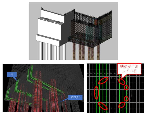
図-3 橋梁下部工鉄筋の配筋照査
